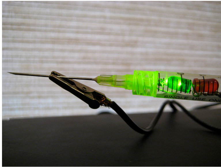
Figure 6. Medical syringe repurposed as an electrical probe
