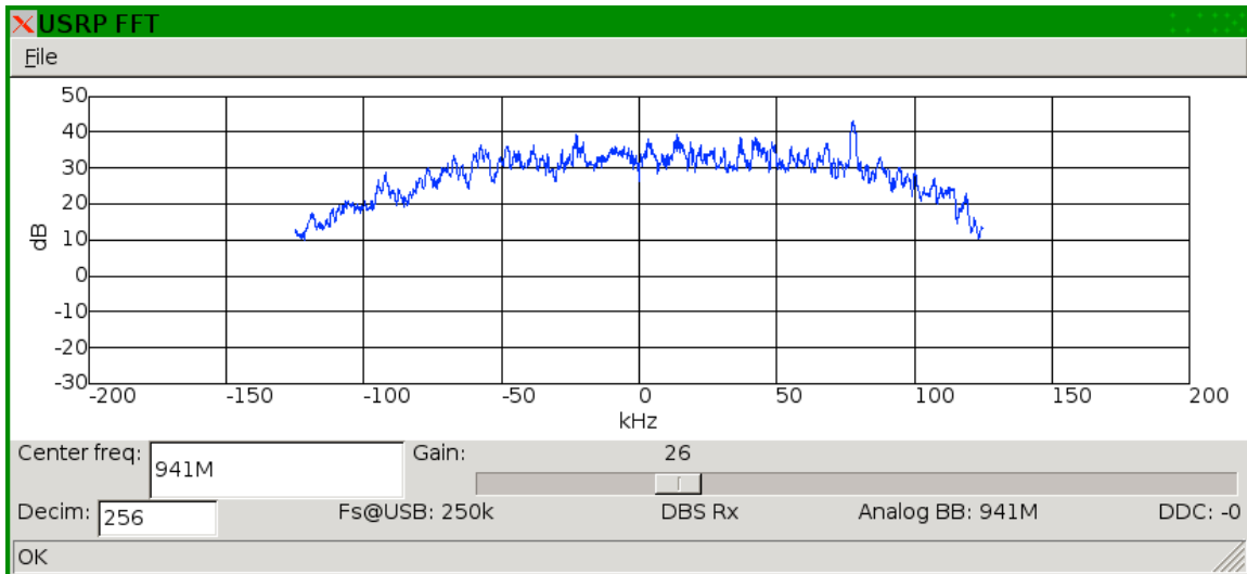
Figure 9. USRP FFT Display
