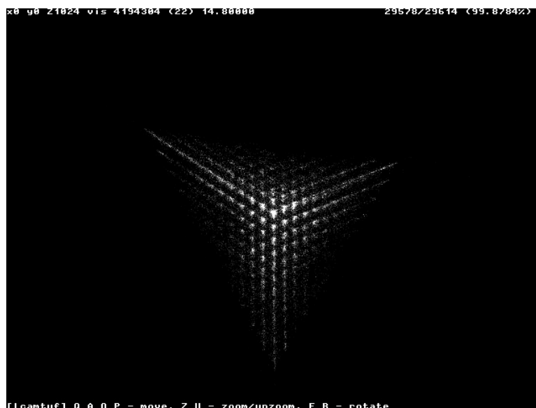
Figure 12. Random number charting indicating a weak RNG
