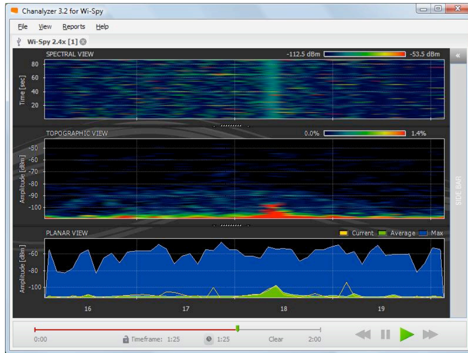
Figure 7. Wi-Spy representation of RF activity at 2.4 GHz
