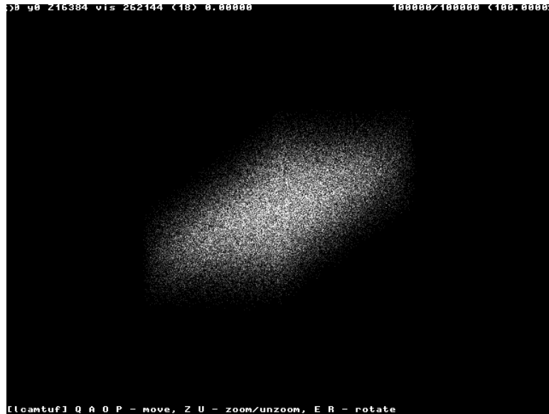
Figure 13. Random number chart indicating a well-distributed RNG
