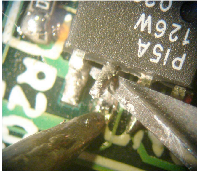
Figure 16. Lifting the Chip Enable Pin
