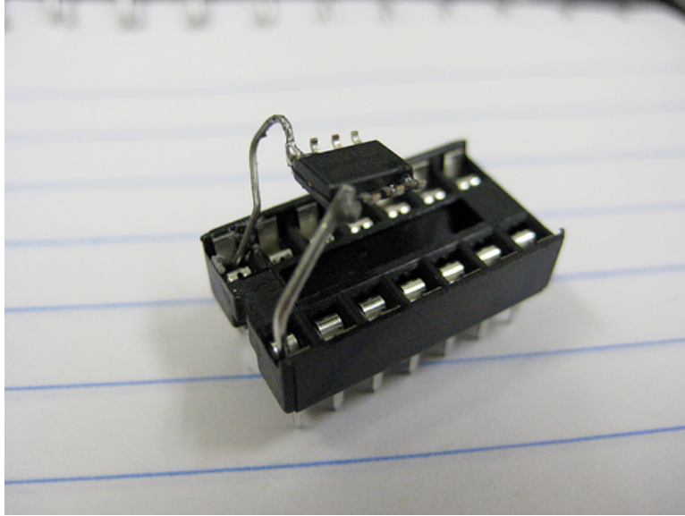
Figure 15. Extracted EEPROM Connected to ZIF Socket
