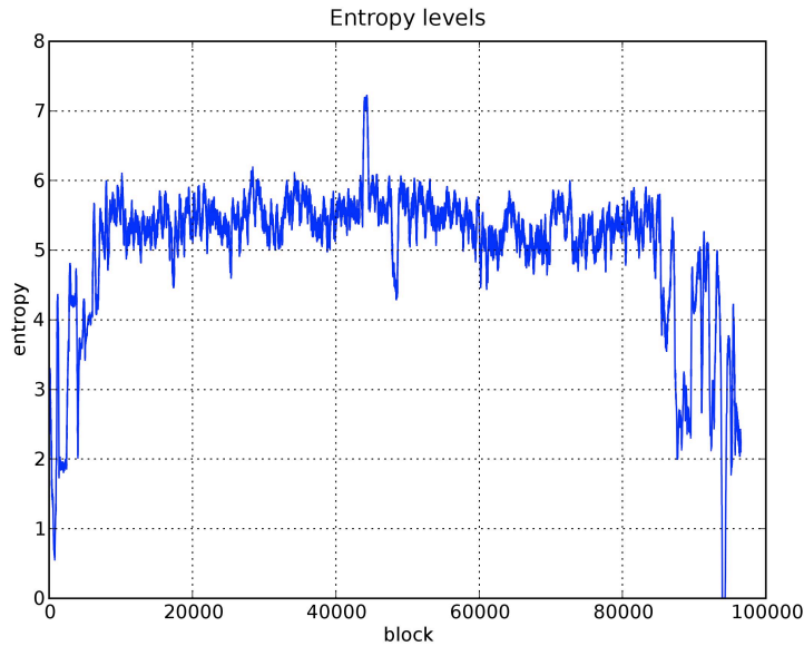
Figure 19. Entropy visualization for an example binary
