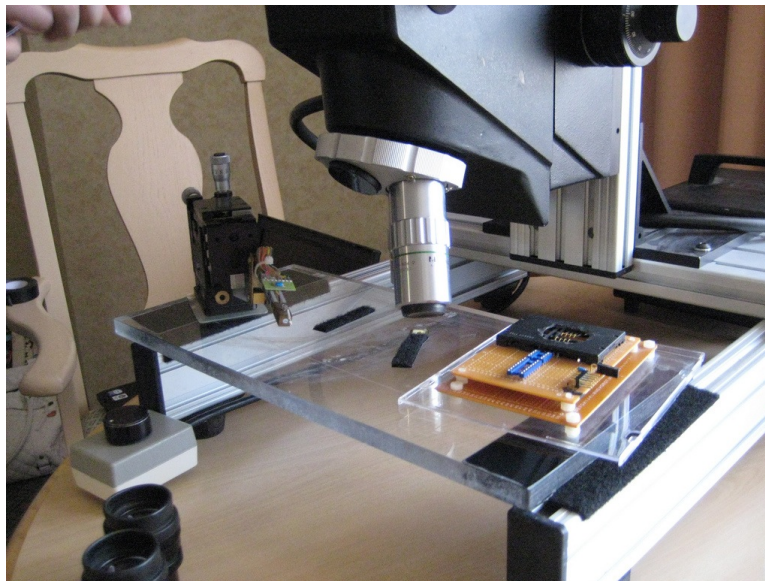
Figure 17. Flylogic Engineering's portable probe station
