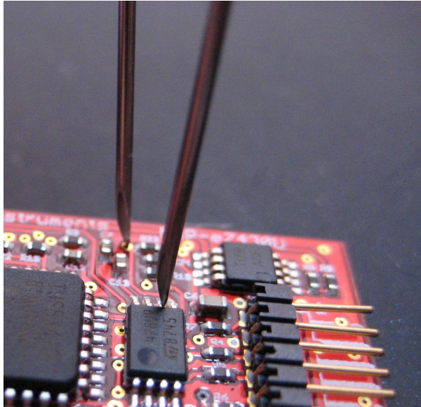
Figure 11. Snooping an I 2 C bus.
