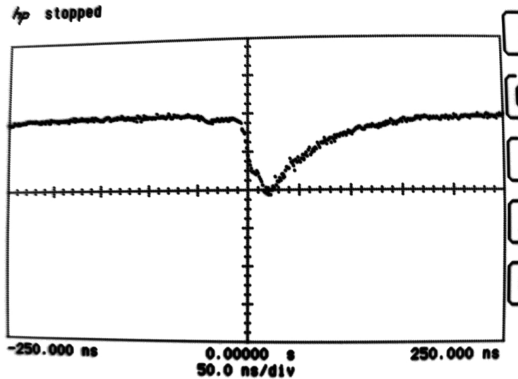
Figure 5. An oscilloscope's view of a voltage-glitching attack.
